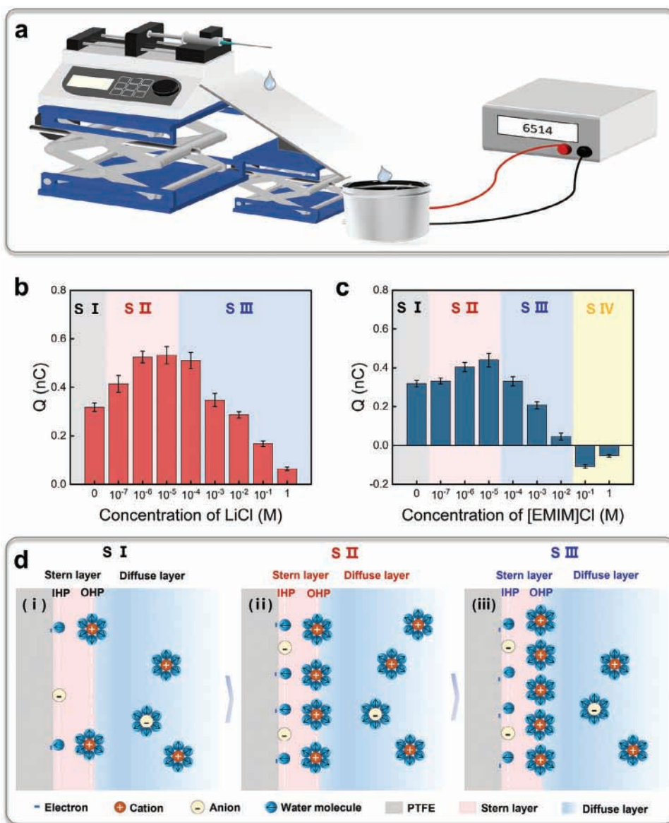
Figure 2. Droplet triboelectric charge controlled by EDL regulation. a) Experimental setup diagram for measuring the triboelectric charge of the droplets. b) Triboelectric charges measured in LiCl solutions of different concentrations. c) Triboelectric charges measured in [EMIM]Cl solution of different concentrations. d) Mechanism of formation of the EDL at the CE interface between droplets and PTFE film. (i) EDL structure for stage I. (ii) EDL structure for stage II. (iii) EDL structure for stage III.
