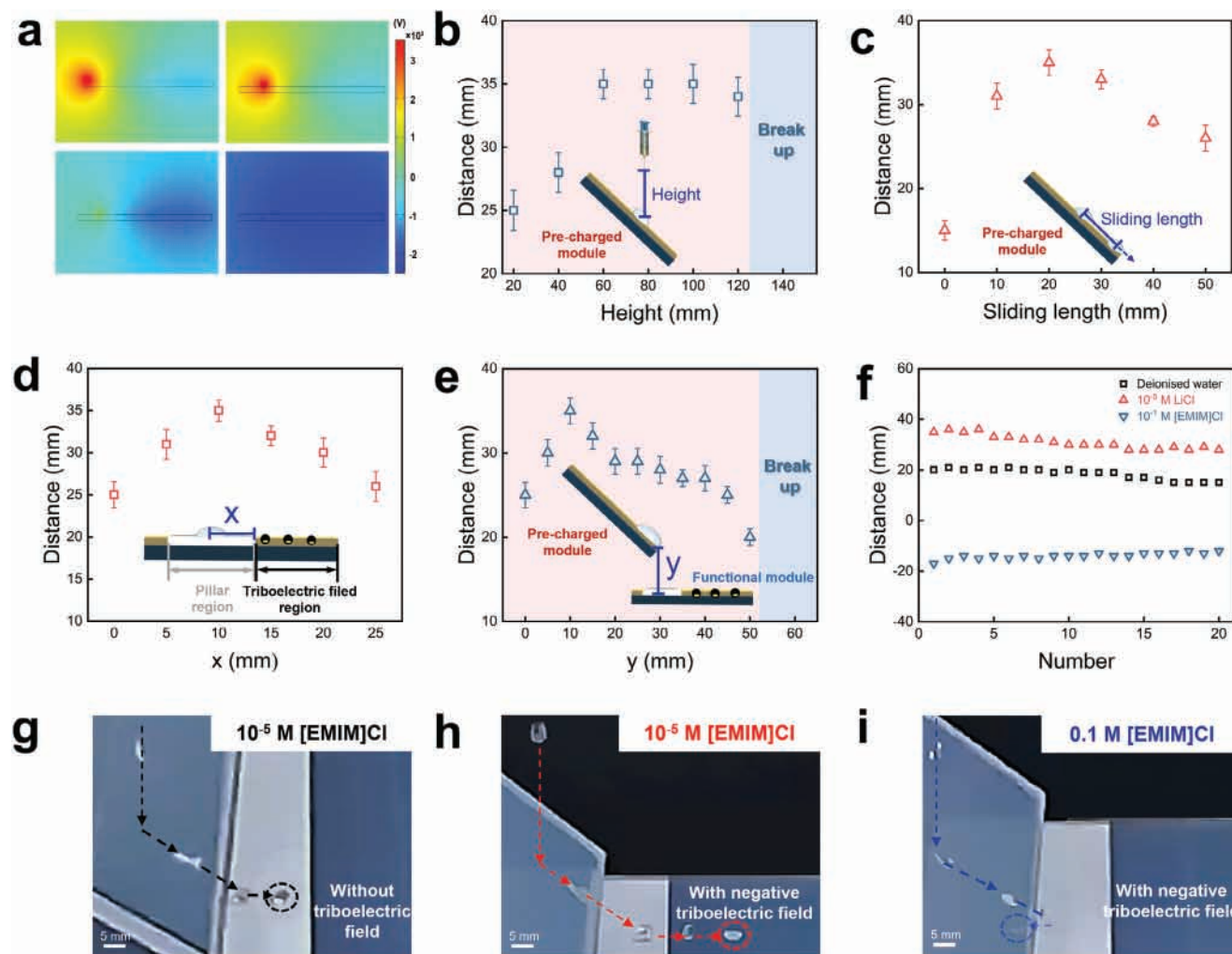
Figure 3. Performance characterization of droplet manipulation. a) Simulation of the surface potential distribution of PTFE during droplet motion. b) Effect of droplet release height on the pre-charged module on its motion distance on the functional module. c) Effect of droplet sliding length on the pre-charged module on its motion distance on the functional module. d) Effect of the length between the droplet's landing point in the micrometer-sized pillar region and the triboelectric field region on its motion distance. e) Effect of the height from the functional module surface to the horizontal plane of the pre-charged module edge on droplet motion distance. f) Property changes of droplet motion after driving 20 droplets consecutively. g) A 10^{-5} M [EMIM]Cl droplet was slid from the pre-charged module to the functional module with no triboelectric field. h) A 10^{-5} M [EMIM]Cl droplet was slid from the pre-charged module to the functional module with a negative triboelectric field. i) A 0.1 M [EMIM]Cl droplet was slid from the pre-charged module to the functional module with a negative triboelectric field. The error bars in a, b, d, and e were standard error values of three tests.
