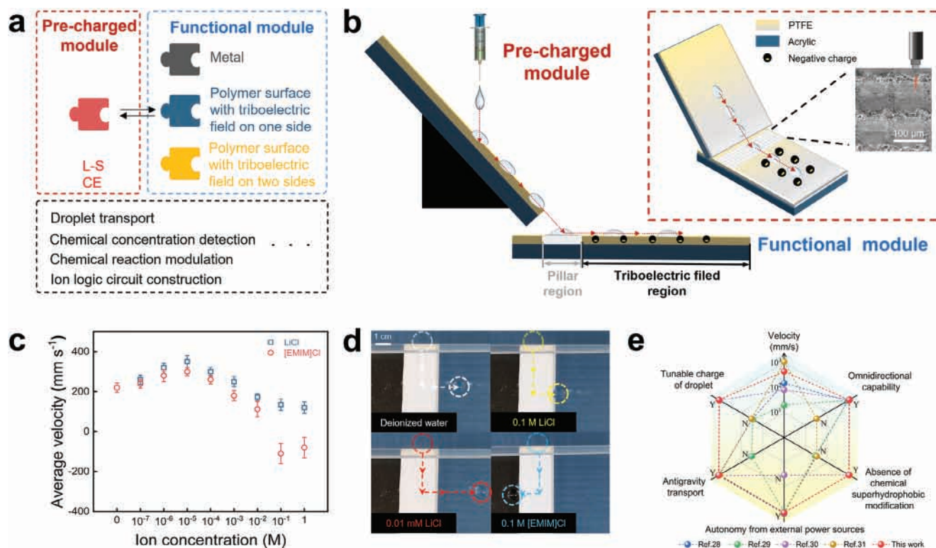
Figure 1. Plug-and-play triboelectric droplet manipulation. a) Schematic diagrams showed that Plug-and-play was usually assembled from two basic modules (pre-charged, functional module). b) Schematic detail of the modular droplet manipulation device. c) The average velocity of movement of LiCl and [EMIM]Cl droplets of different concentrations on the surface of a negative triboelectric field. The error bars were standard error values of three tests. d) Deionized water, 10^{-5} M LiCl, 0.1 M LiCl, and 0.1 M [EMIM]Cl droplets could be classified according to their direction of motion and distance. e) Comparison of our work with previously reported electrically based droplet manipulation from six perspectives (velocity, omnidirectional capability, absence of chemical superhydrophobic modification, autonomy from external power sources, antigravity transport, and tunable charge of droplet). “Y” and “N” denoted Yes and No, respectively.
